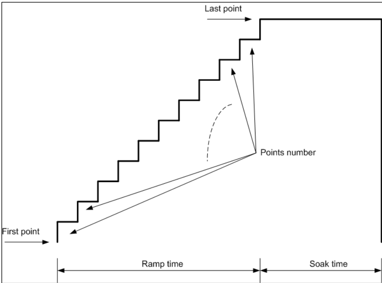
Figure 58 – Ramp profile
